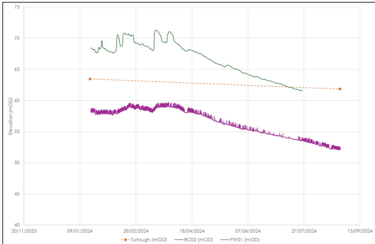
Figure 7.6: Groundwater Level Monitoring Hydrographs
