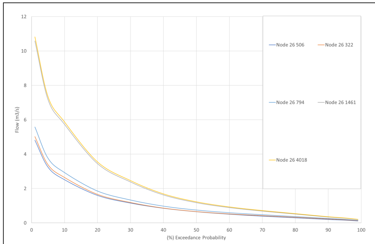
Figure 7.2: River Flow Exceedance Curves
